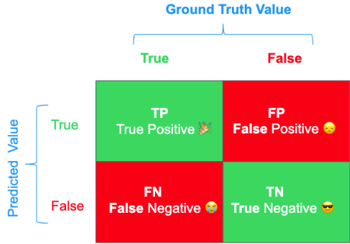
Gambar 6.5 Confusion Matrix
